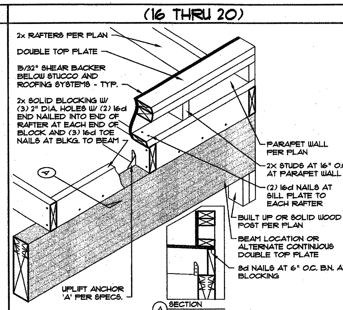
16 CONNECTION RAFTER TO BEAM AT WALK DECK SCALE: 1" = 1'-0" © 8D5-05-04 BAI BAI NO.: 107698AZ
