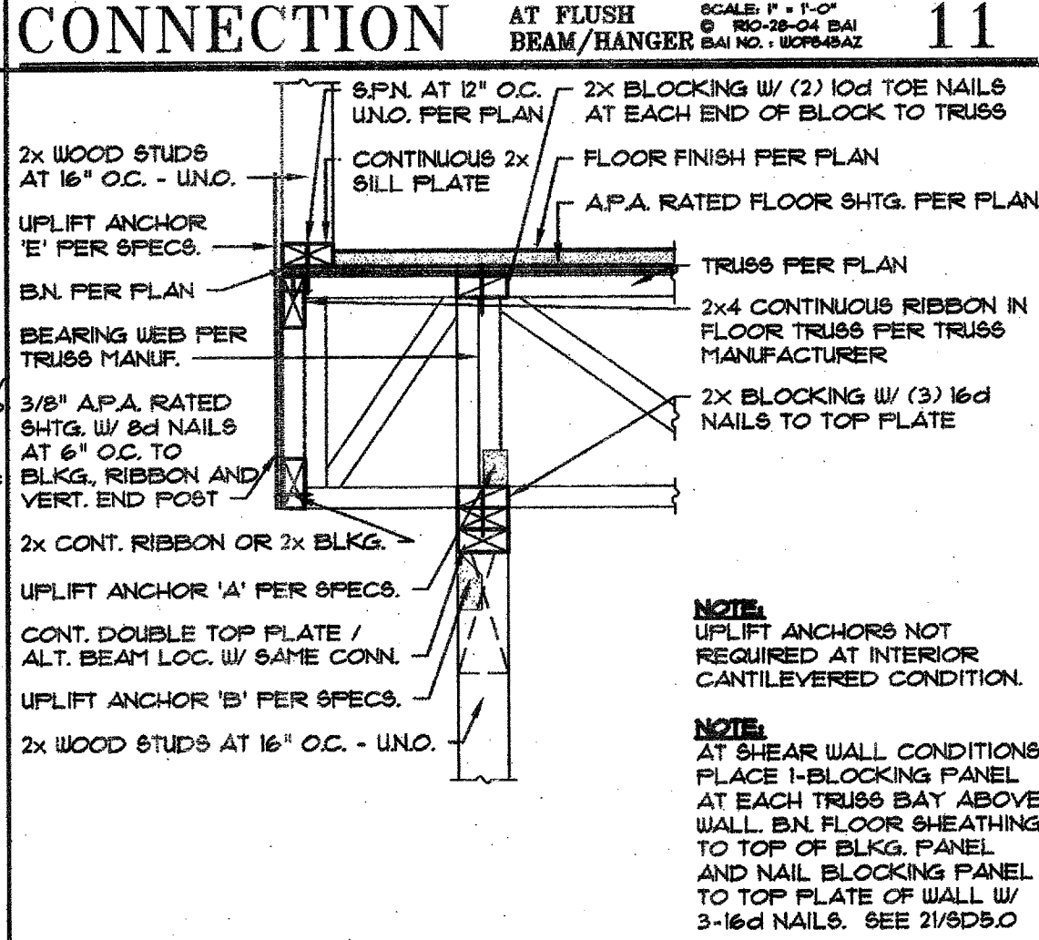
12 CANT. SUPPORT AT EXT. WALL SCALE: 1" = 1'-0" © 8D5-05-04 BAI BAI NO.: 107698AZ
