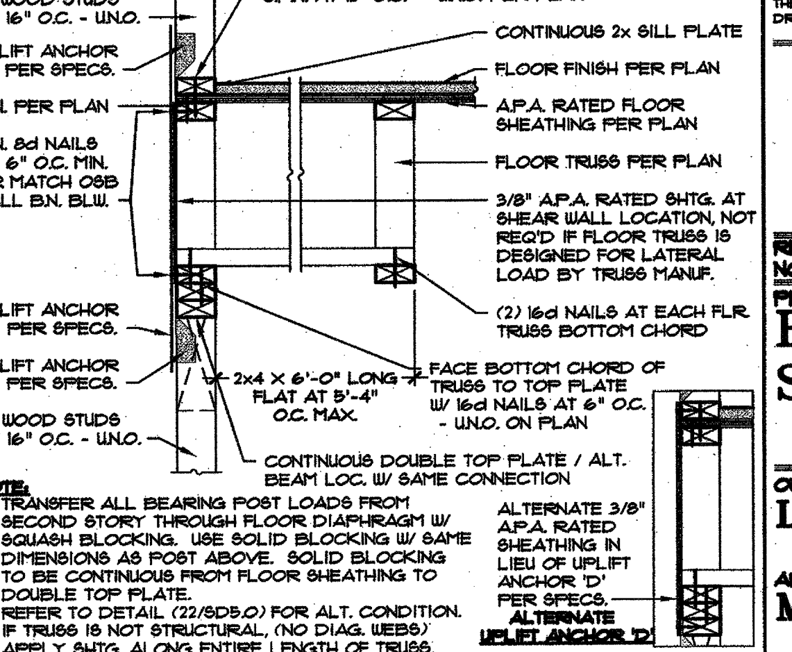
2 RIM AT EXTERIOR WALL PARALLEL SCALE: 1" = 1'-0" © 8D5-05-04 BAI BAI NO.: 107698AZ
