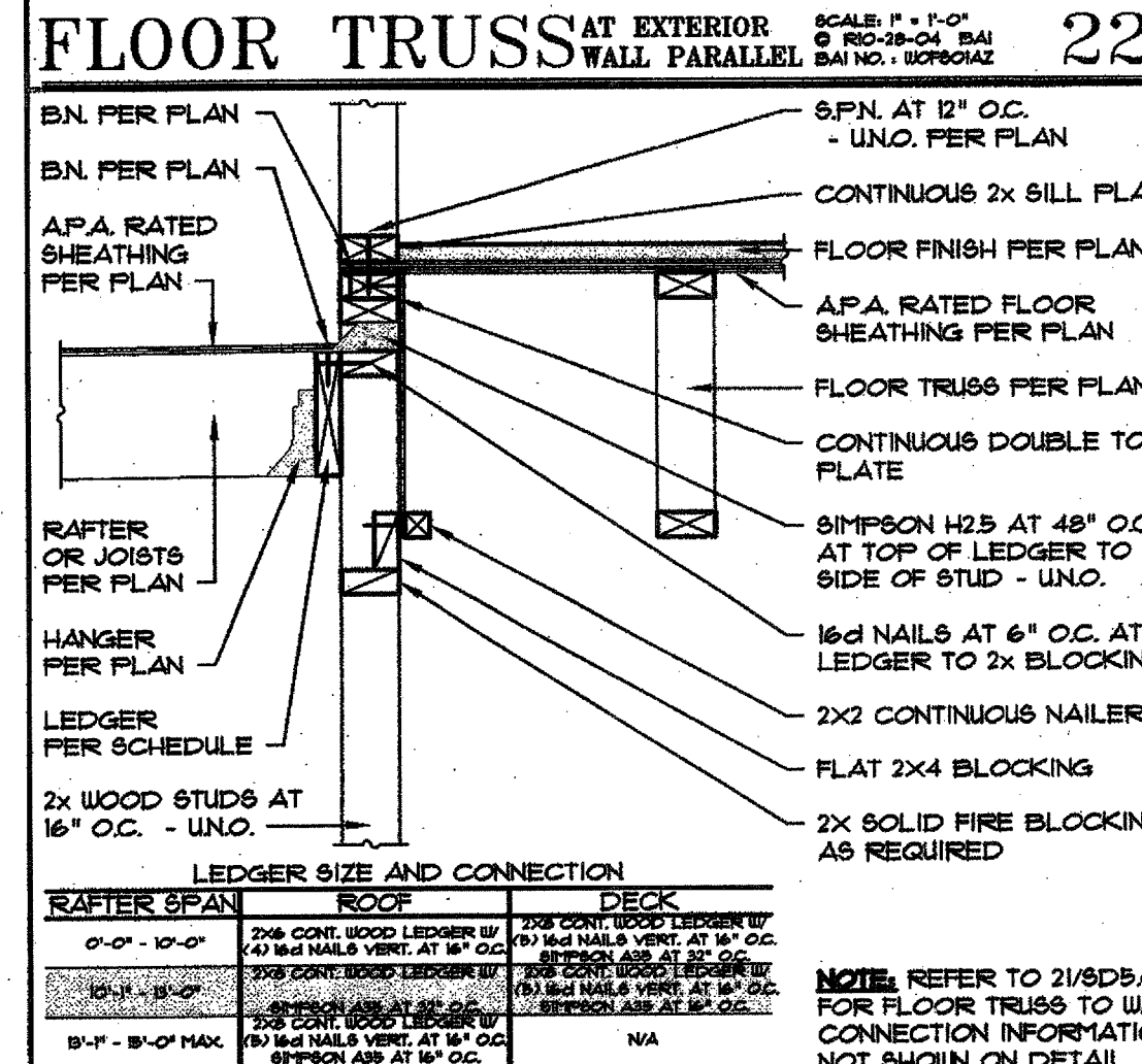
23 FLOOR TRUSS AT LEDGER AT PERP. RAFTER SCALE: 1" = 1'-0" © 8D5-05-04 BAI BAI NO.: 107698AZ
