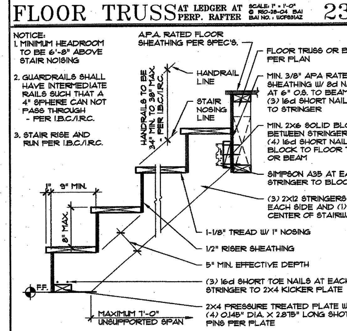
19 STAIR AND LANDING SCALE: 1" = 1'-0" © 8D5-05-04 BAI BAI NO.: 107698AZ
