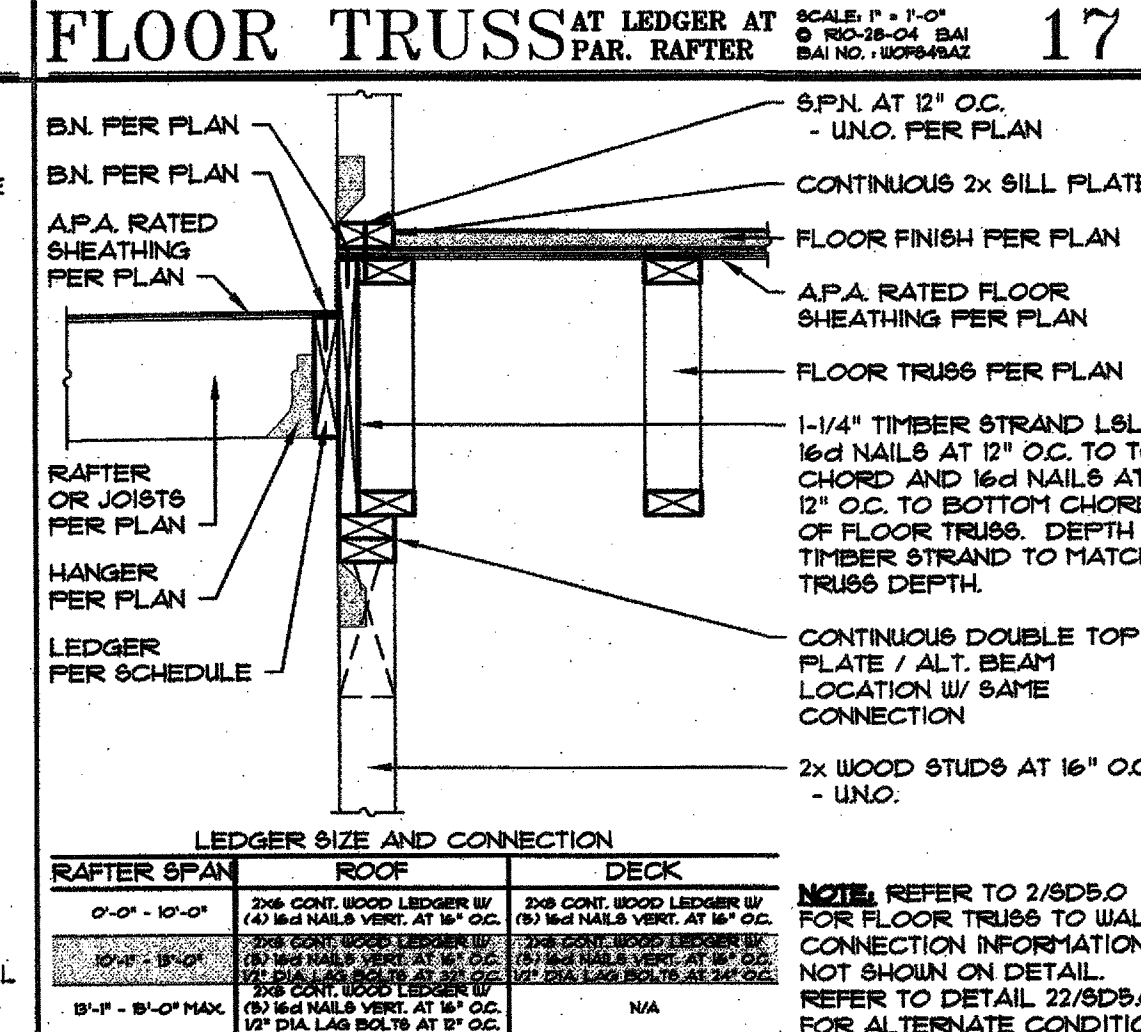
18 FLOOR TRUSS AT LEDGER AT PERP. RAFTER SCALE: 1" = 1'-0" © 8D5-05-04 BAI BAI NO.: 107698AZ
