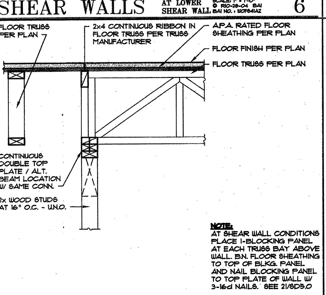
7 INT. SUPPORT PERP. TO WALL SCALE: 1" = 1'-0" © 8D5-05-04 BAI BAI NO.: 107698AZ
