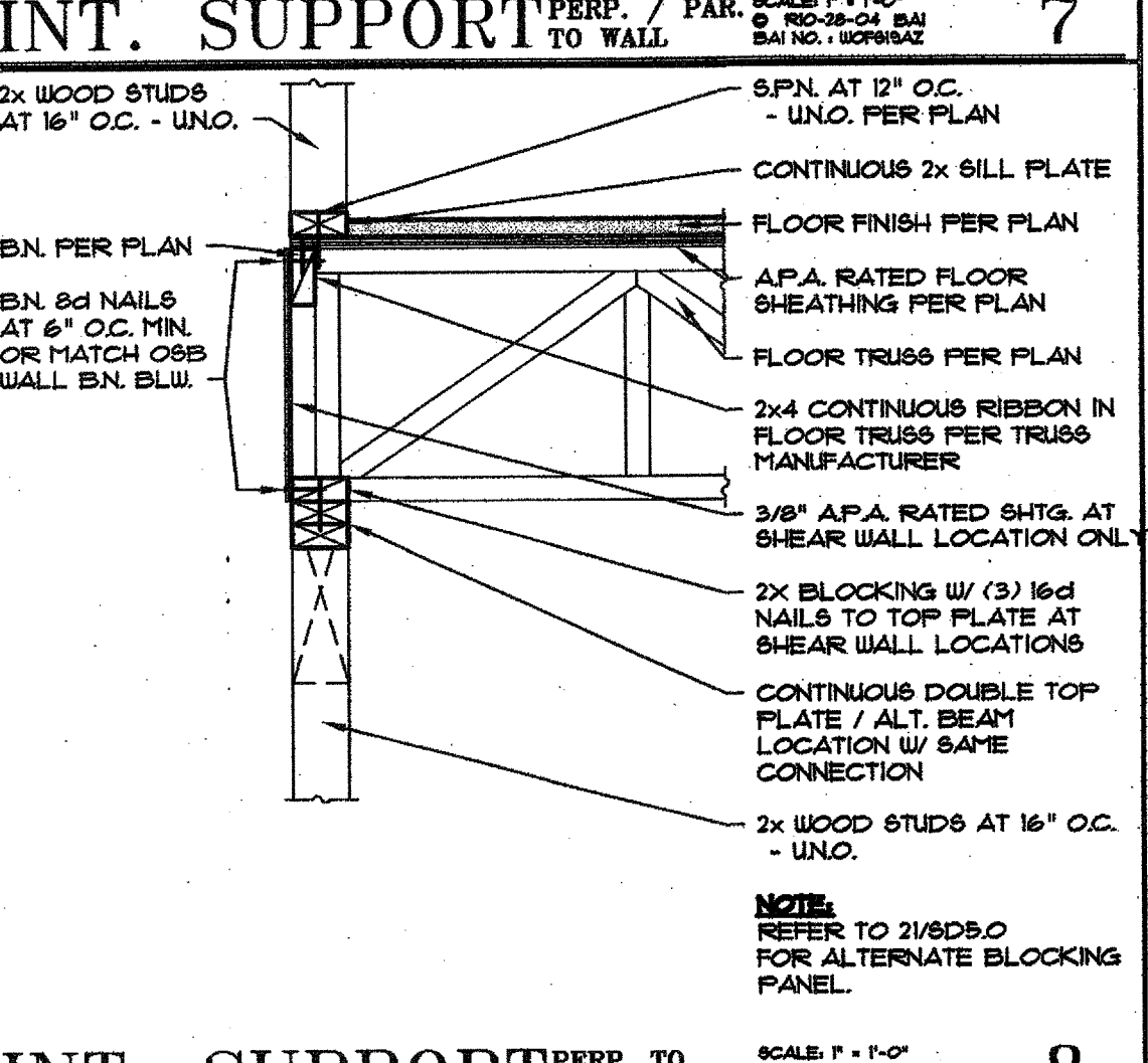
8 INT. SUPPORT PERP. TO WALL SCALE: 1" = 1'-0" © 8D5-05-04 BAI BAI NO.: 107698AZ
