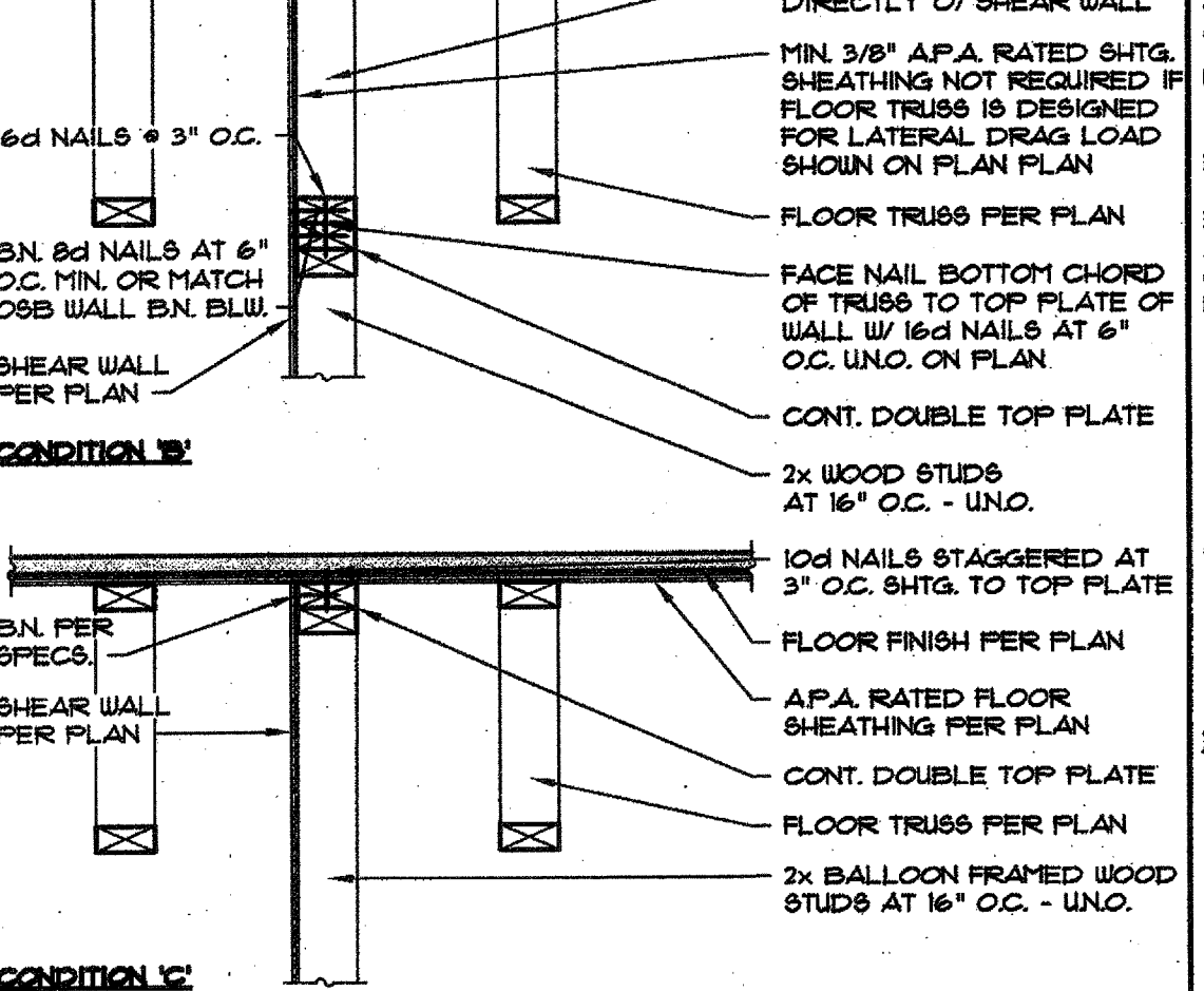
6 SHEAR WALLS AT LOWER SHEAR WALL SCALE: 1" = 1'-0" © 8D5-05-04 BAI BAI NO.: 107698AZ
