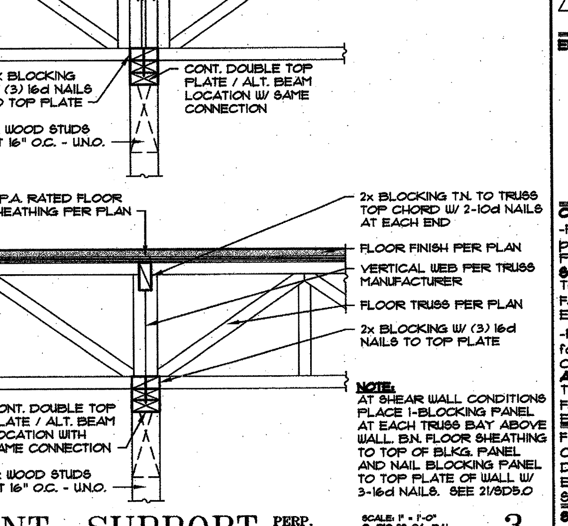
3 INT. SUPPORT PERP. TO WALL SCALE: 1" = 1'-0" © 8D5-05-04 BAI BAI NO.: 107698AZ
