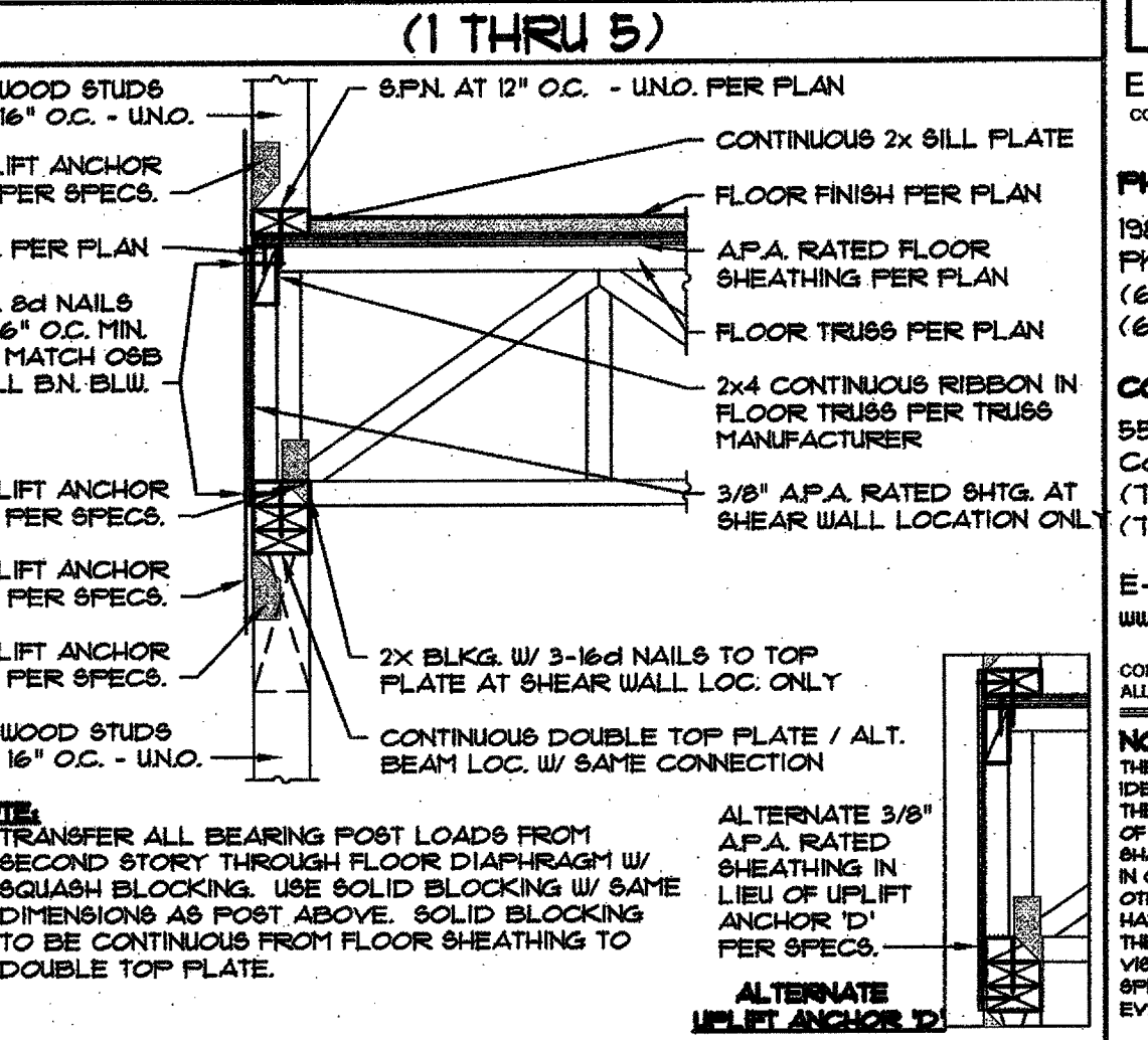
1 RIM AT EXTERIOR WALL PERPENDICULAR SCALE: 1" = 1'-0" © 8D5-05-04 BAI BAI NO.: 107698AZ
