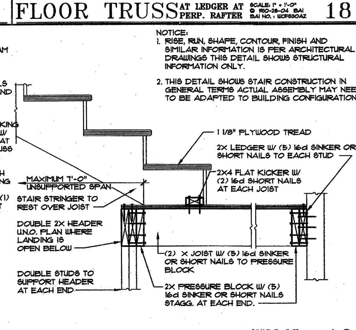
19 STAIR AND LANDING SCALE: 1" = 1'-0" © 8D5-05-04 BAI BAI NO.: 107698AZ
