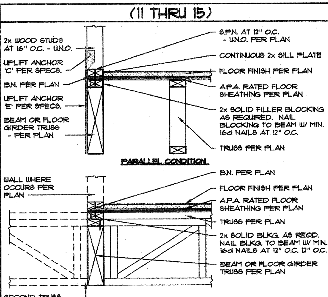
11 CONNECTION AT FLUSH BRAM/HANGER SCALE: 1" = 1'-0" © 8D5-05-04 BAI BAI NO.: 107698AZ
