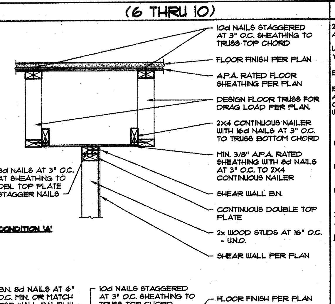
6 SHEAR WALLS AT LOWER SHEAR WALL SCALE: 1" = 1'-0" © 8D5-05-04 BAI BAI NO.: 107698AZ
