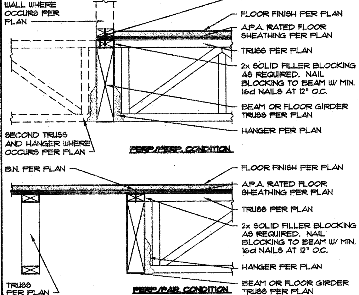
11 CONNECTION AT FLUSH BRAM/HANGER SCALE: 1" = 1'-0" © 8D5-05-04 BAI BAI NO.: 107698AZ
