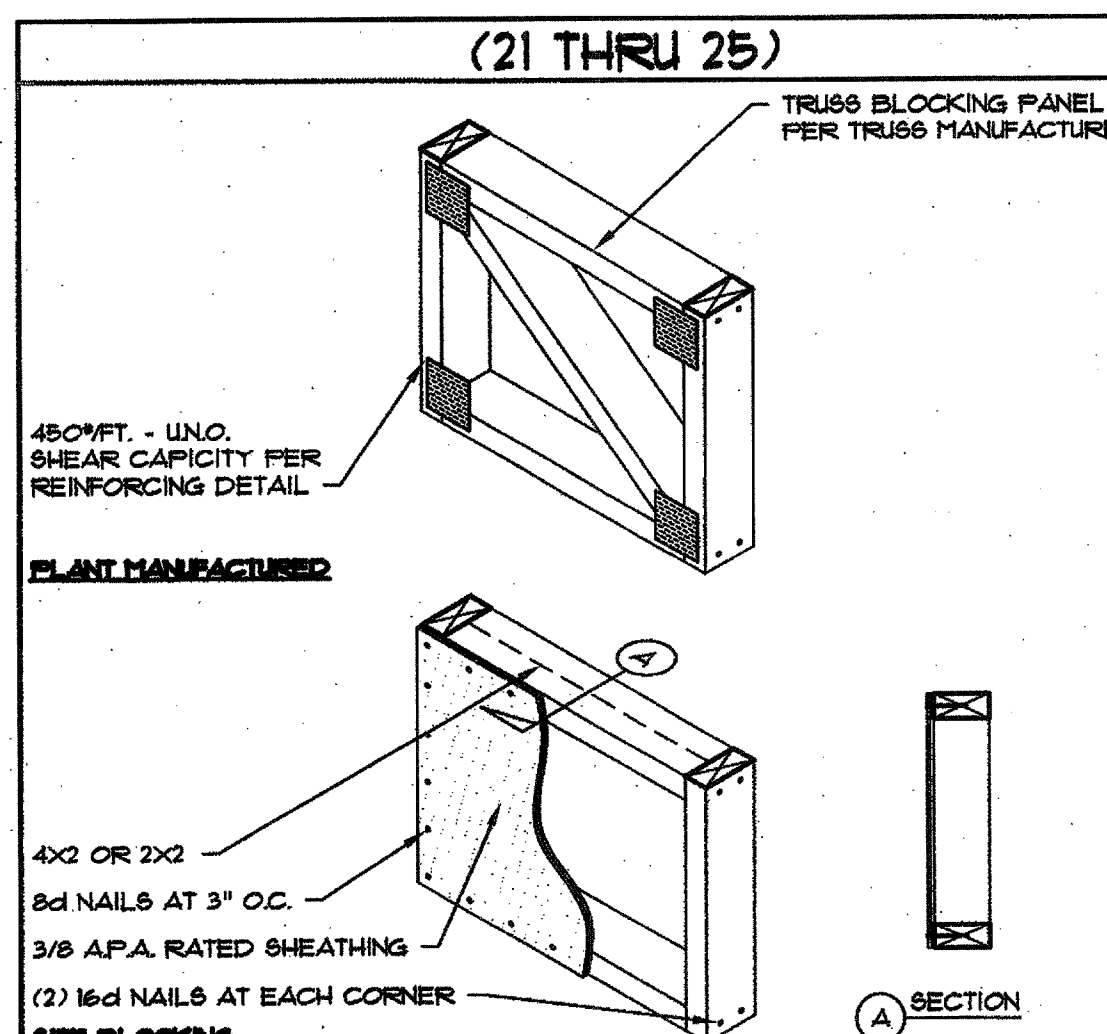
21 BLOCKING PANEL SCALE: 1" = 1'-0" © 8D5-05-04 BAI BAI NO.: 107698AZ
